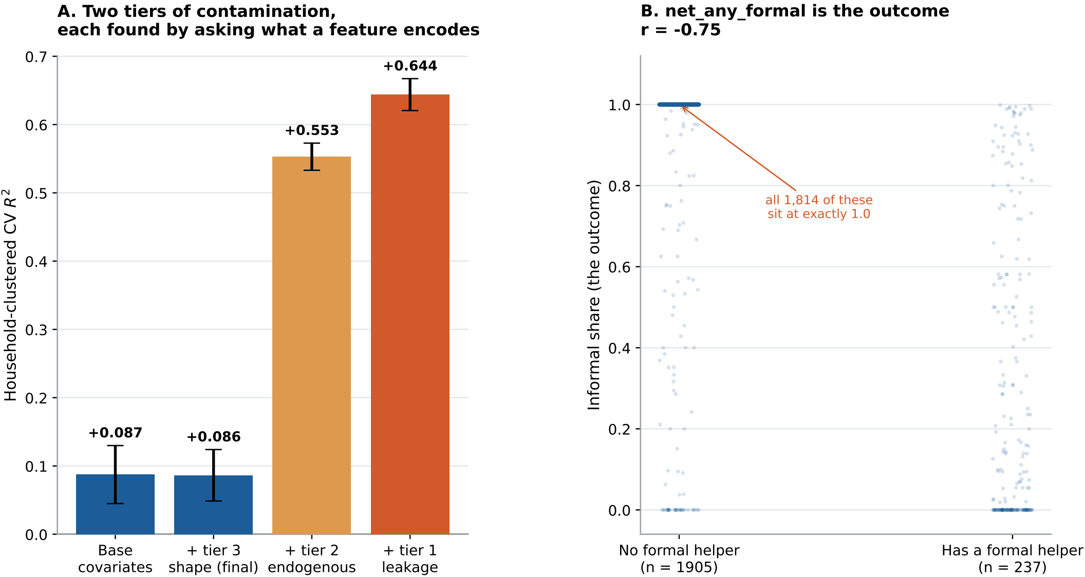
Figure 11. A target-leakage trap, sprung deliberately and then removed
