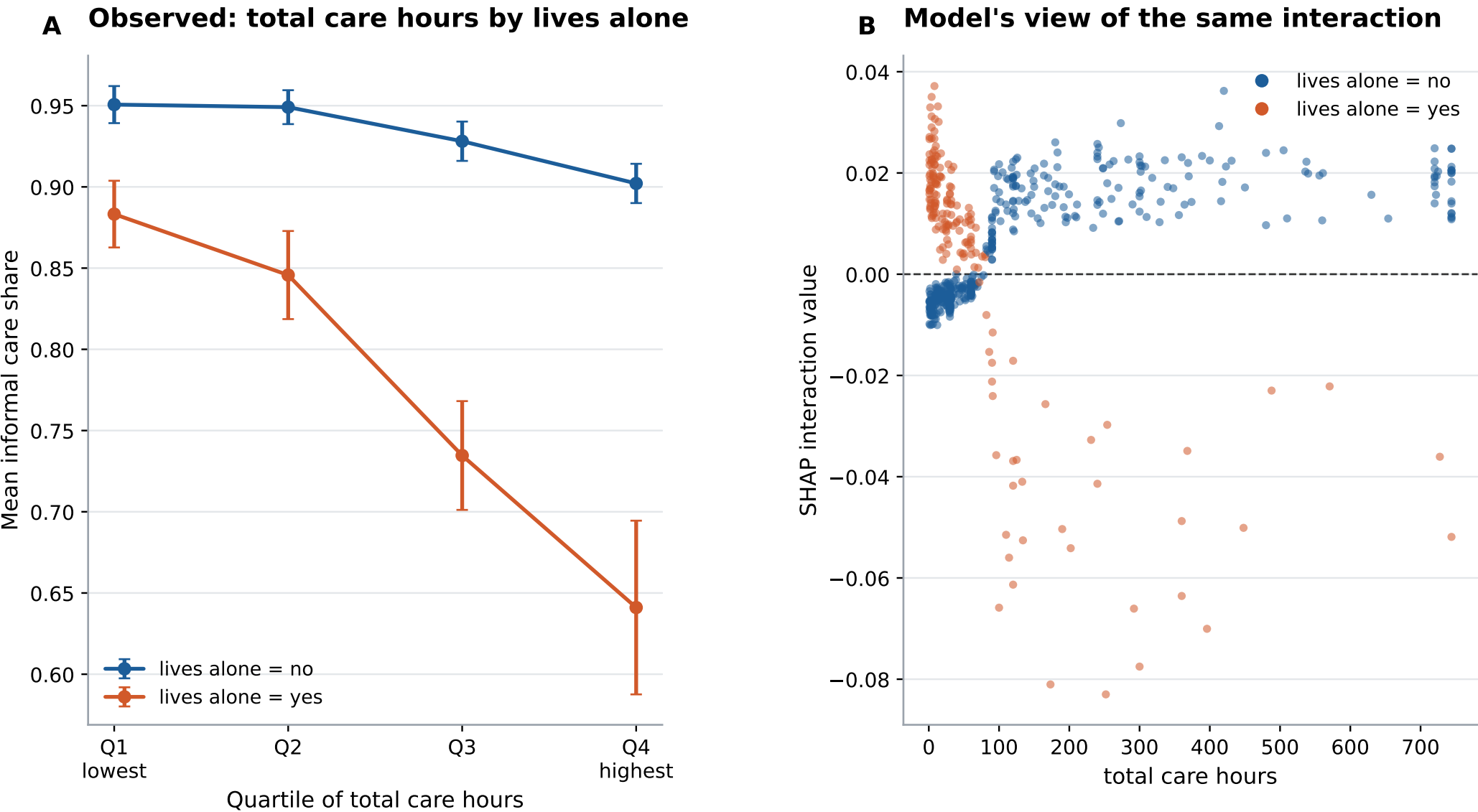
Figure 16. Strongest interaction: total care hours × lives alone ( \beta = -0.032 , p = 0.005 )
