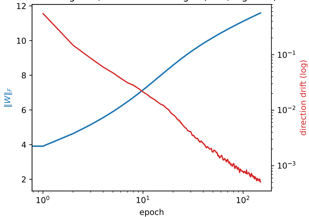
B. Norm grows; direction converges (drift, log axes)
