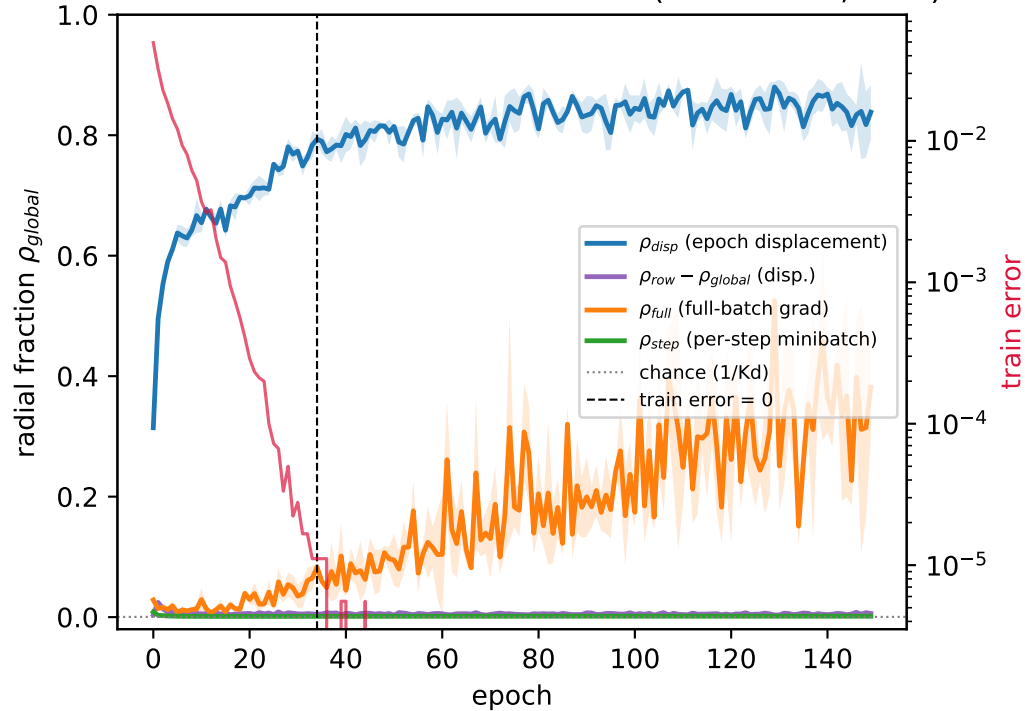
A. Radial fraction: three estimators (MNIST MLP, SGD)
