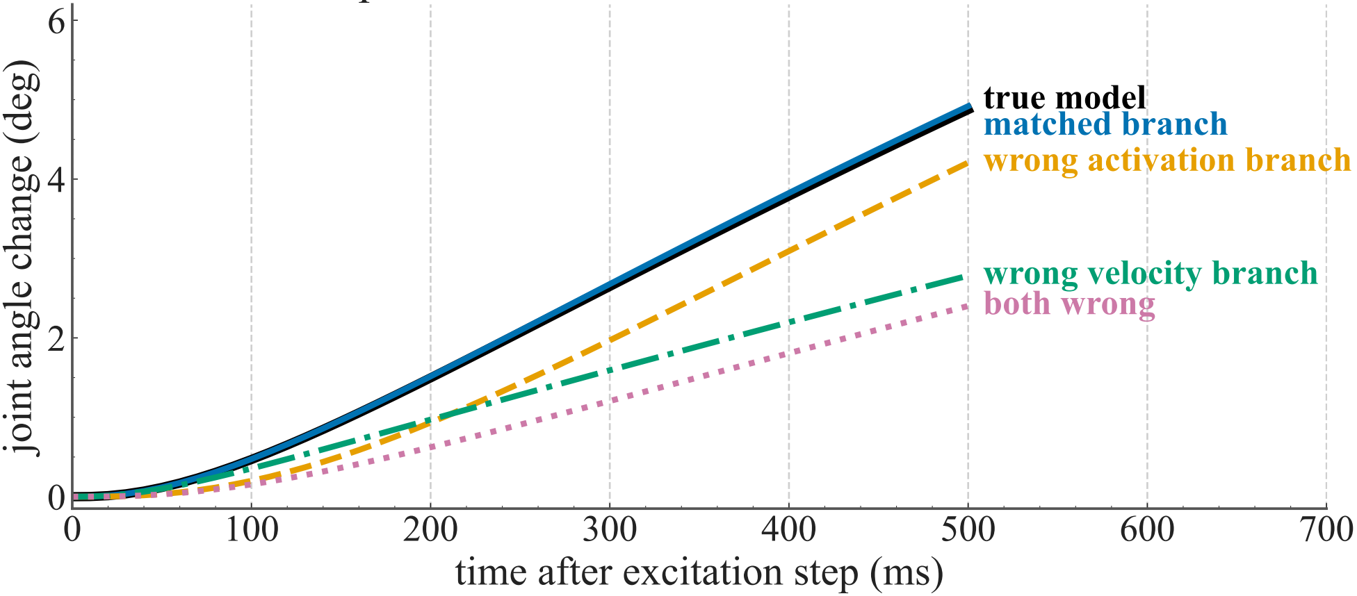
One-shot linear predictions vs the true model
