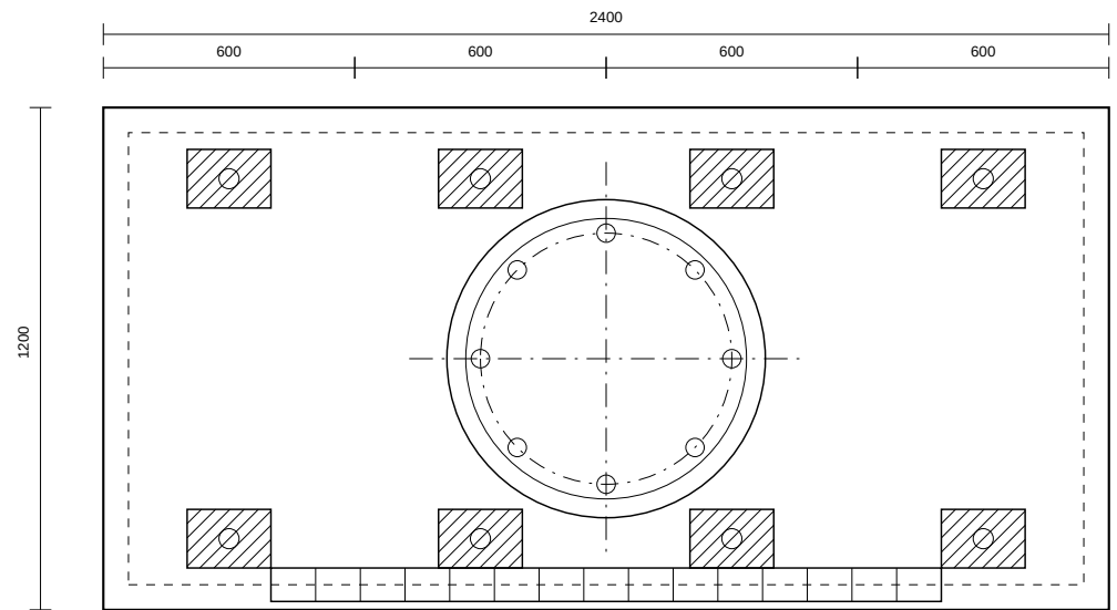
SAMPLE MACHINE BASE - scale 1:20 - dimensions in mm
