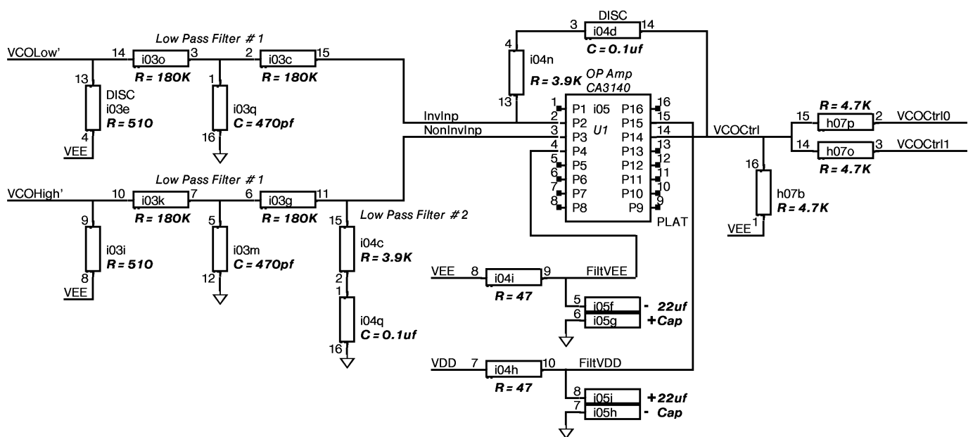
Loop Filter and System VCO
