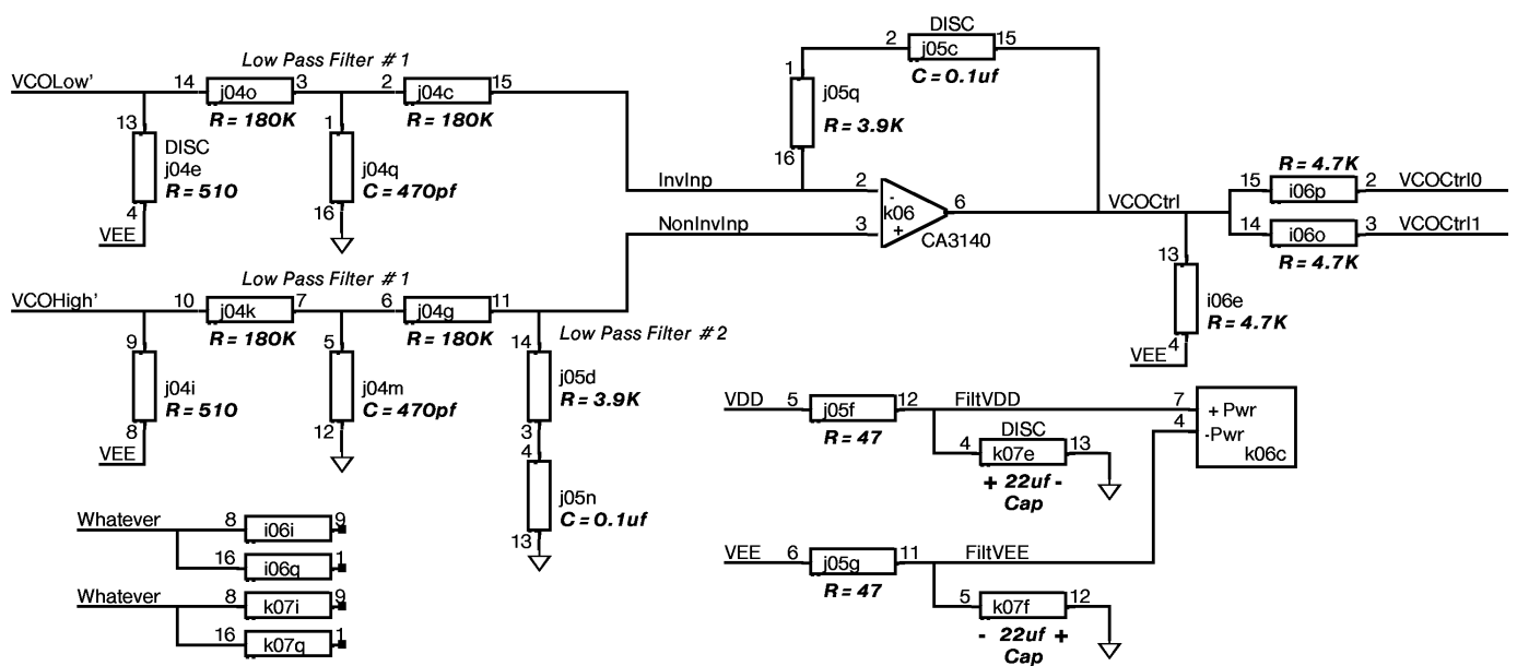
Loop Filter and System VCO
