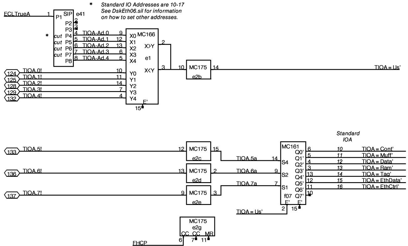
IO Address decoding
