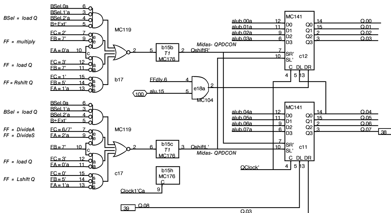
Q Register
