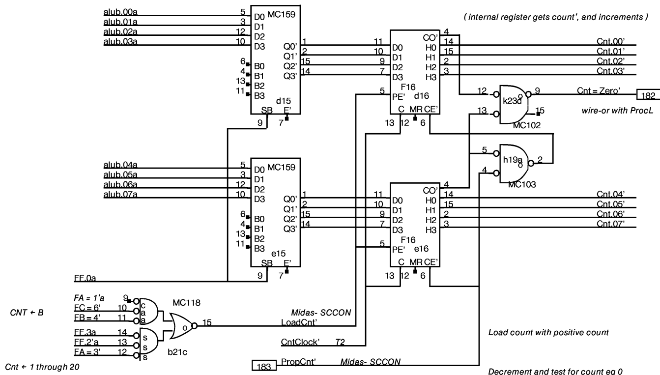
Count Register
