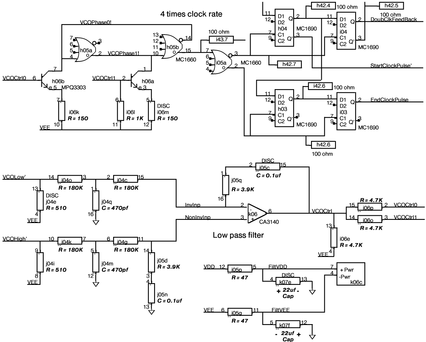
LOOP FILTER AND SYSTEM VCO
