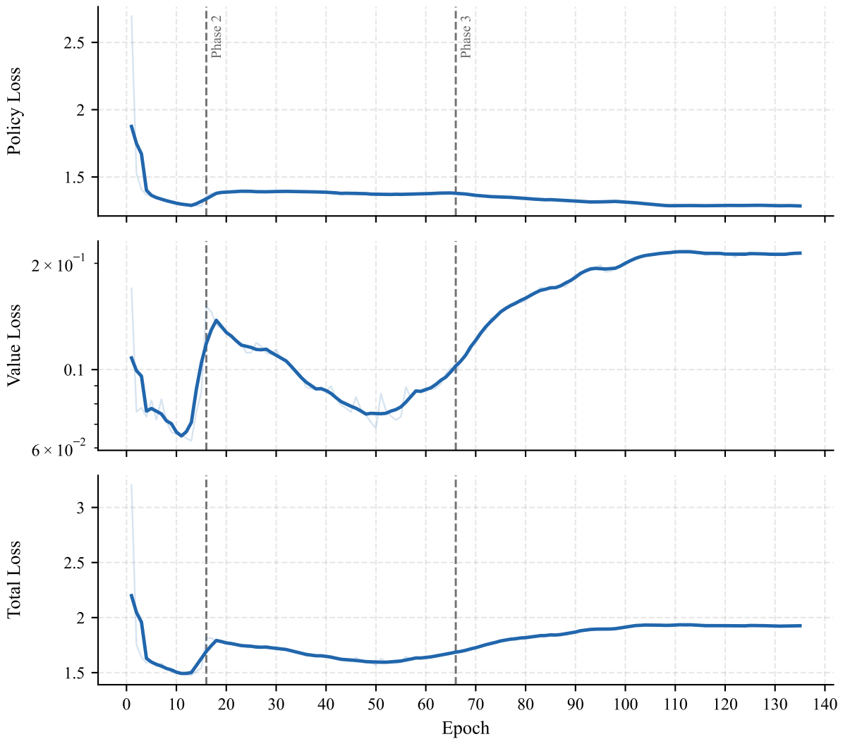
AlphaZero Scalar — Training Loss Curves
