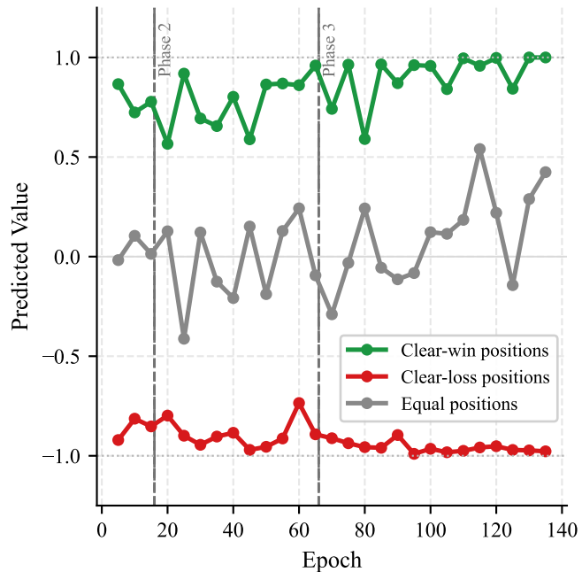
(B) Value Head Calibration
