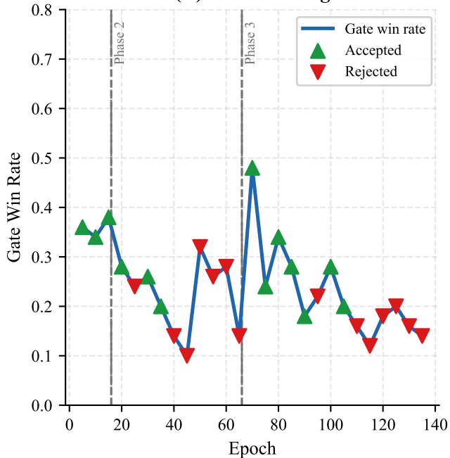
(A) Model Gating
