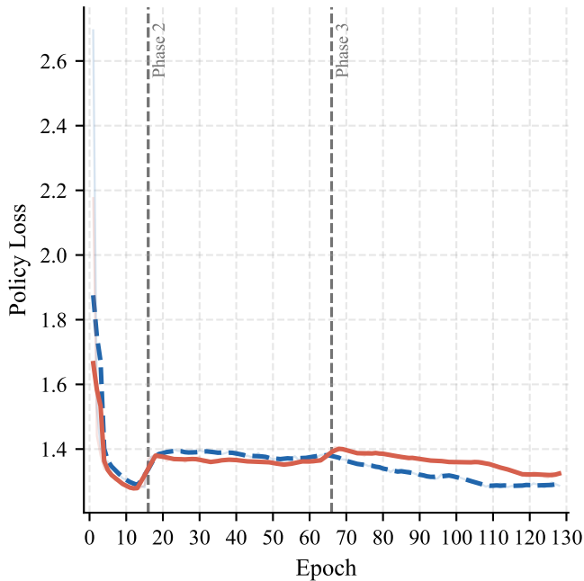
(A) Policy Loss
