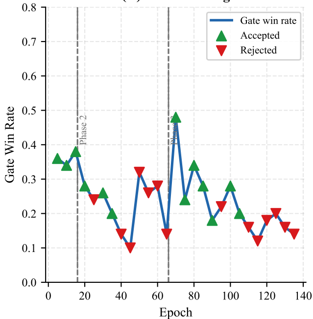
(A) Model Gating
