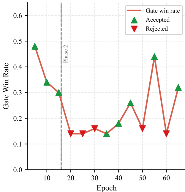
(A) Model Gating
