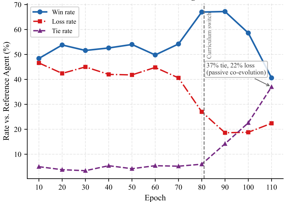
PPO Curriculum — vs. Reference Agent Performance
