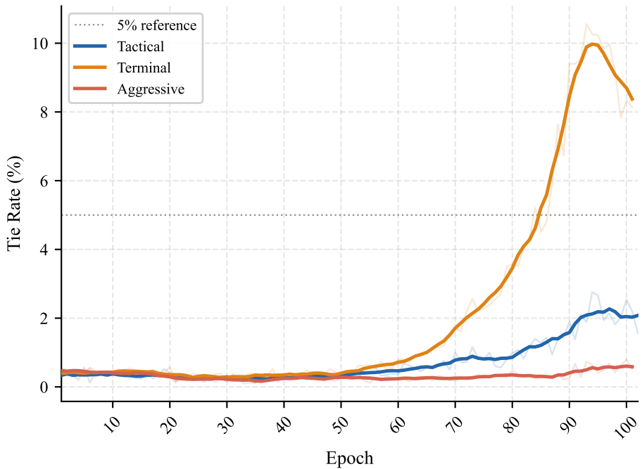
PPO League — Tie Rate by Agent Type
