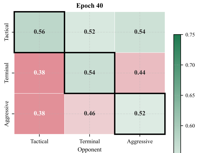
PPO League — Head-to-Head Win Rate Matrix Diagonal (outlined): win rate vs. own checkpoint from 10 epochs prior
