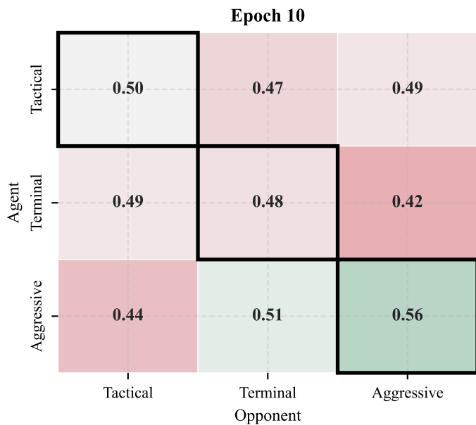
PPO League — Head-to-Head Win Rate Matrix Diagonal (outlined): win rate vs. own checkpoint from 10 epochs prior
