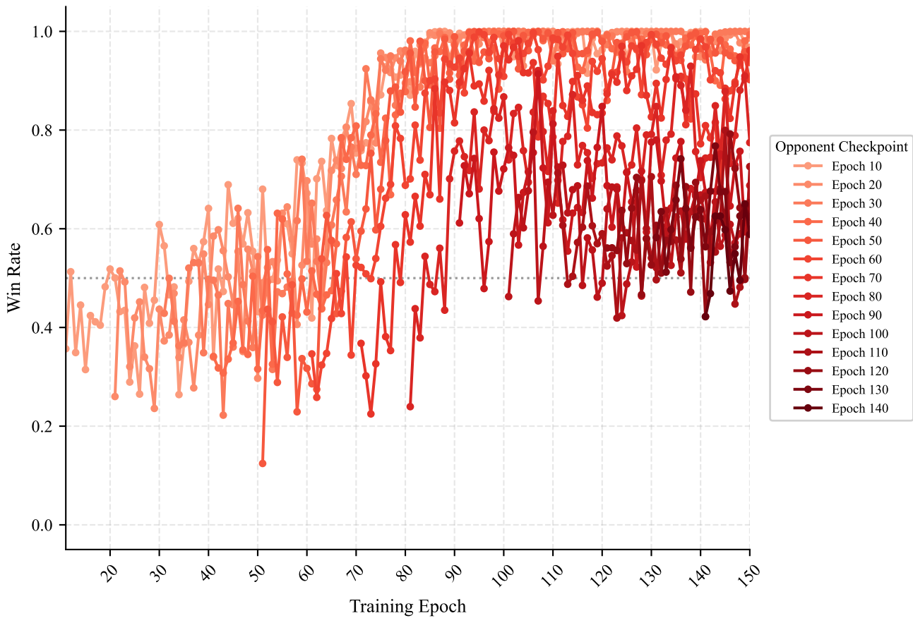
Aggressive Agent vs. Aggressive Opponents
