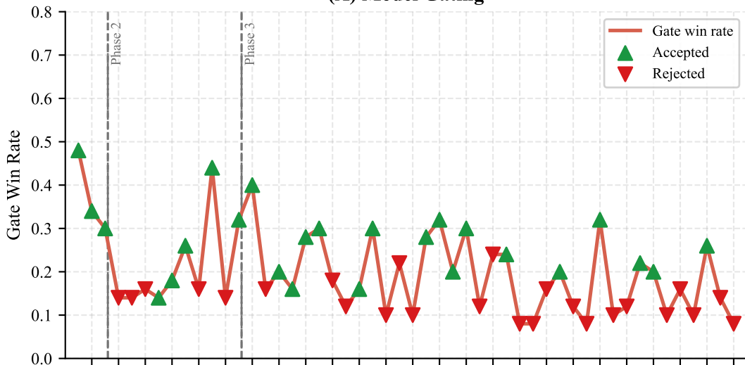
(A) Model Gating
