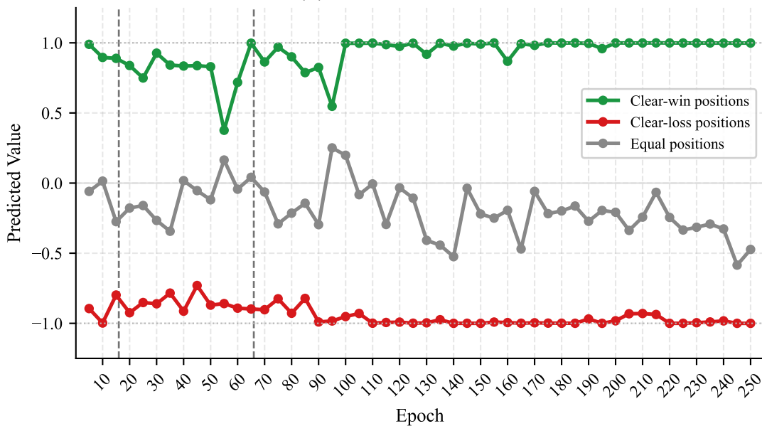
(B) Value Head Calibration
