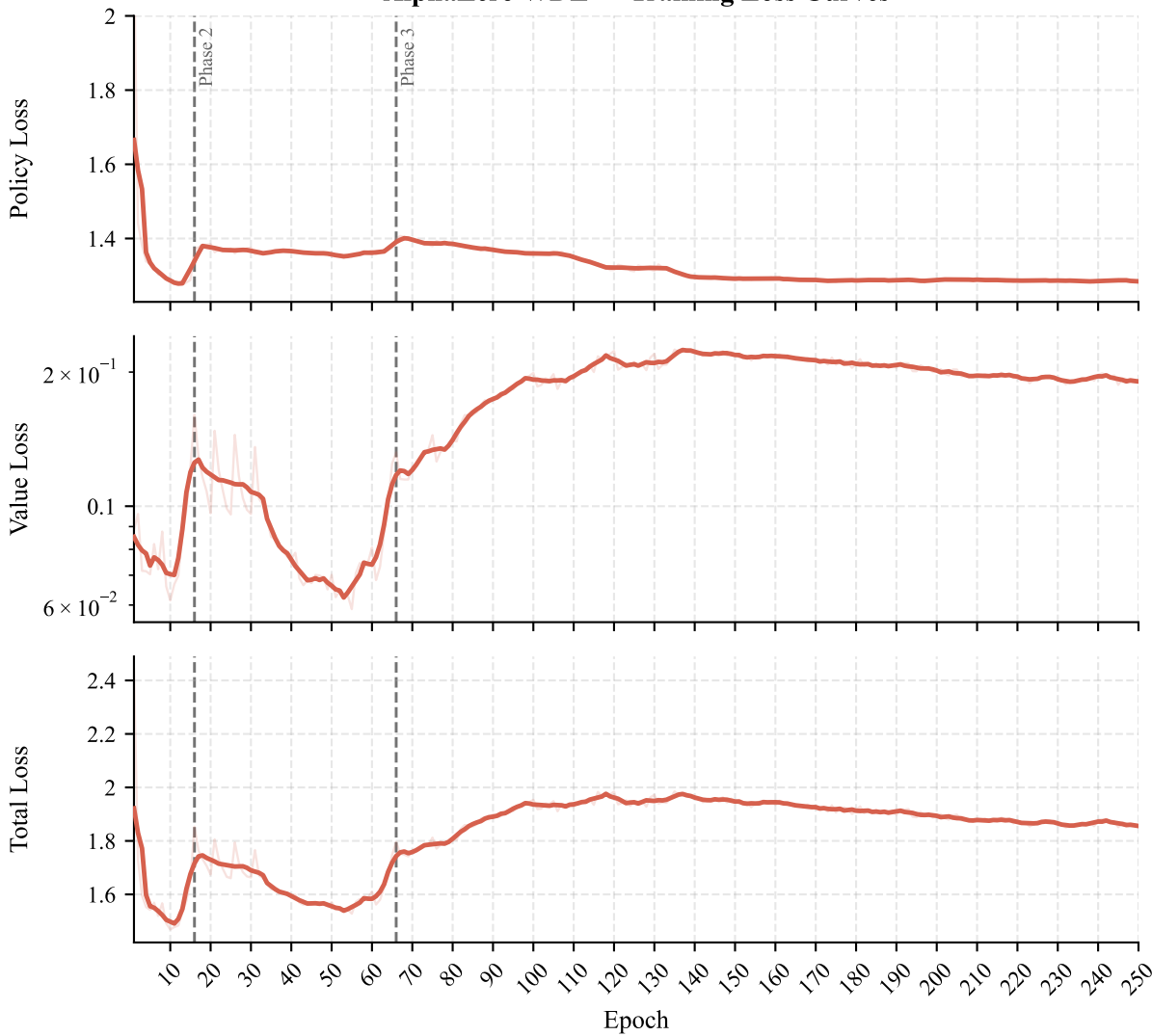
AlphaZero WDL — Training Loss Curves
