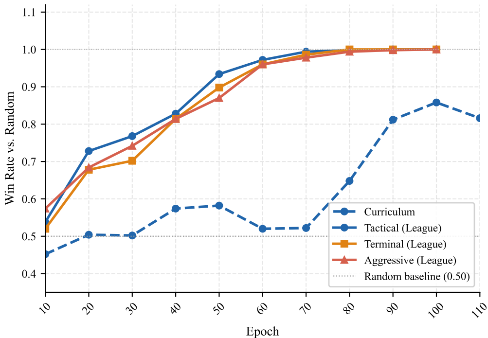
PPO Training Comparison — Win Rate vs. Random Agent
