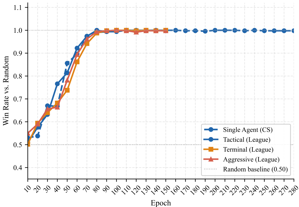
PPO Training Comparison — Win Rate vs. Random
