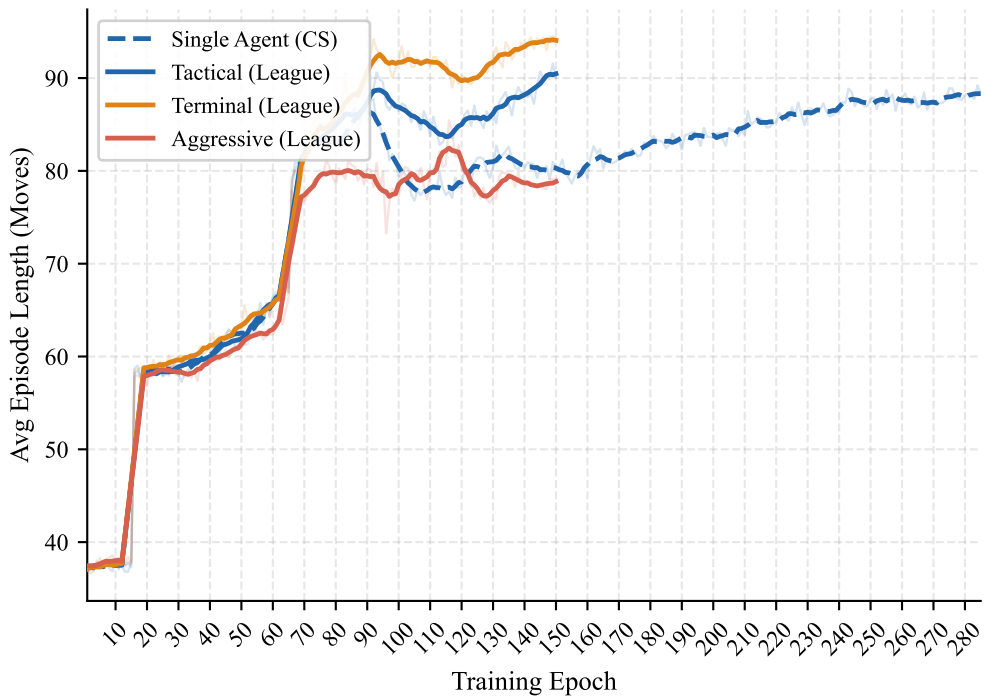
PPO Training Comparison — Episode Length
