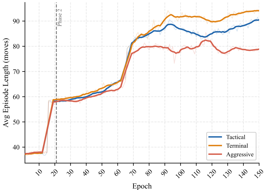
PPO League — Episode Length by Agent Type
