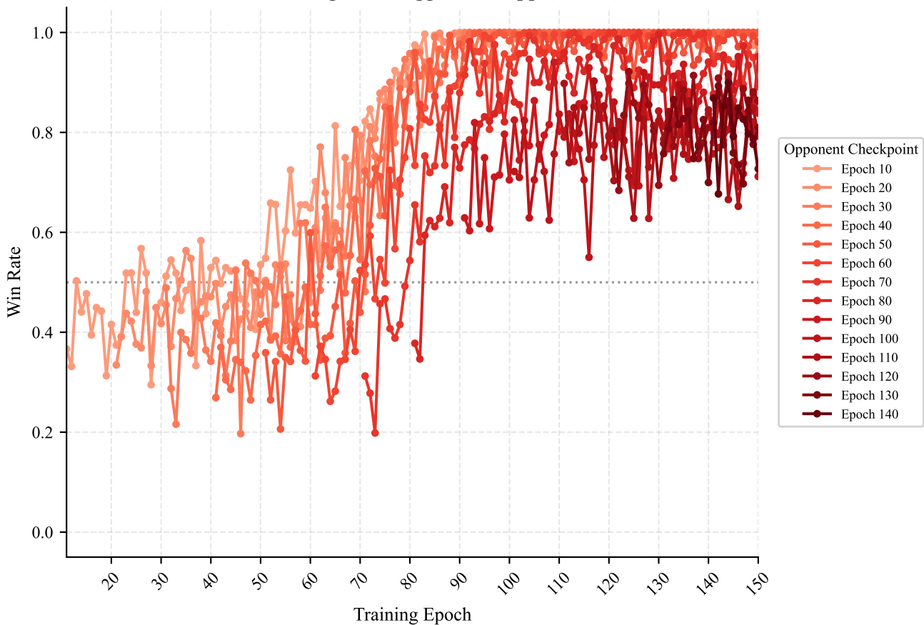
Terminal Agent vs. Aggressive Opponents
