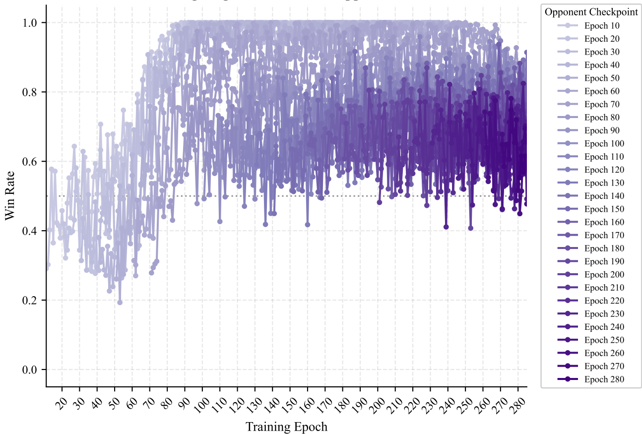
Single Agent vs. Past Pool Opponents
