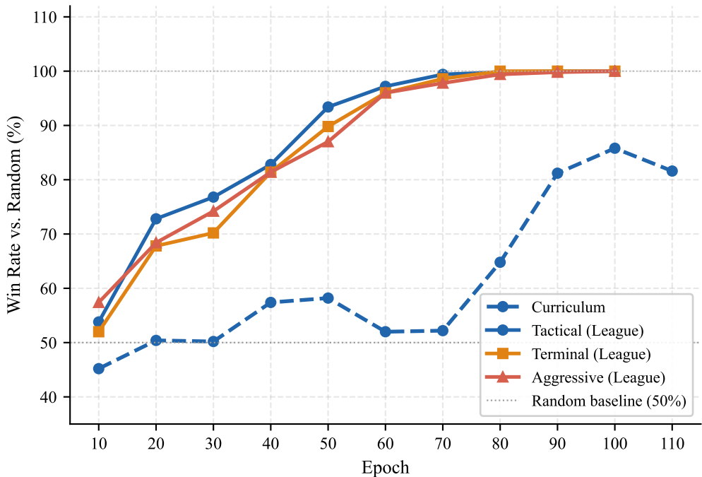
PPO Training Comparison — Win Rate vs. Random Agent
