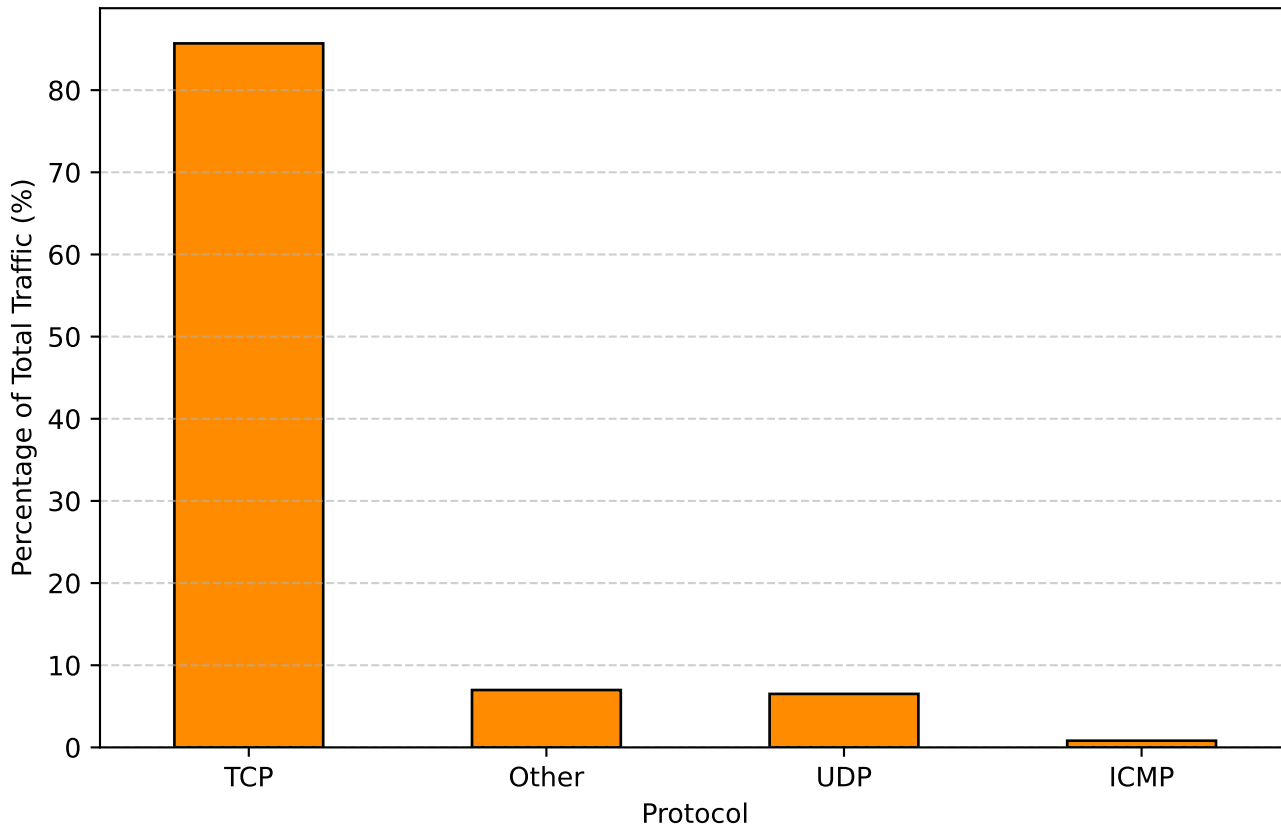
Protocol Breakdown by Data Volume (Bytes)
