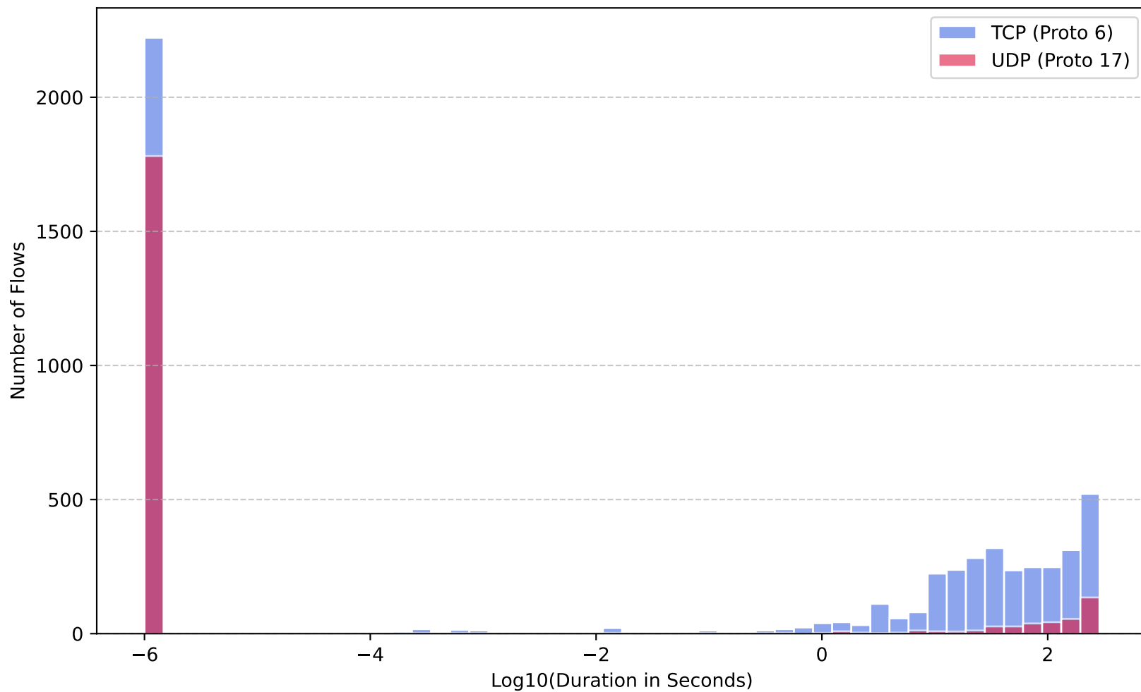
TCP vs UDP Flow Duration Distribution
