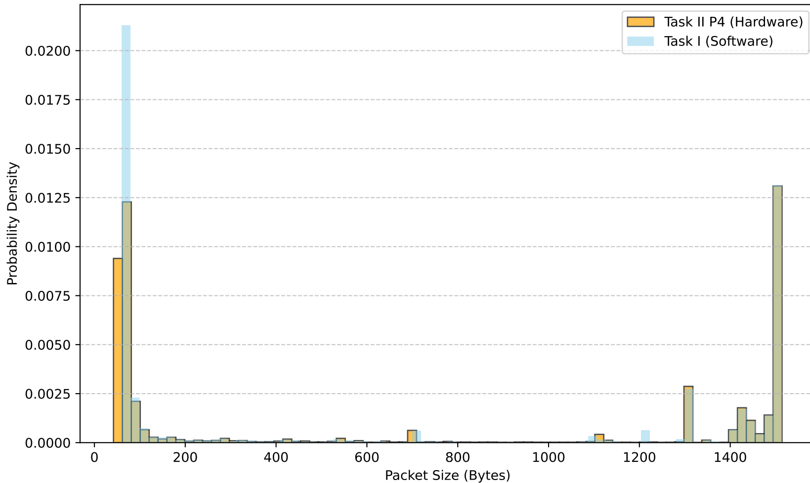
PDF of Packet Sizes (Task I vs Task II)
