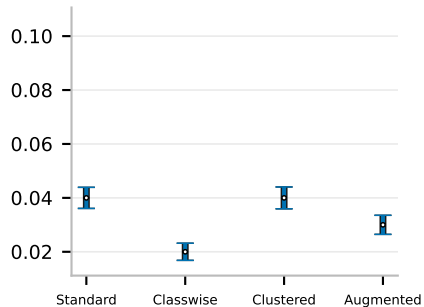
MLP Neural Net (macro F1: 0.61)
