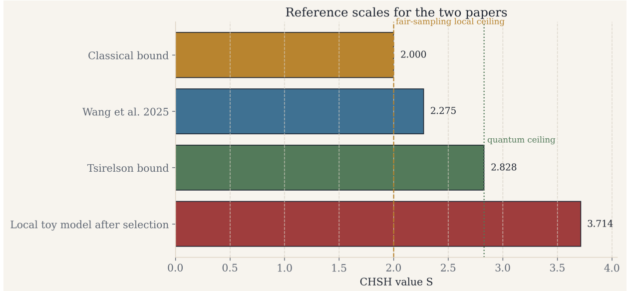
Figure 1: Reference scales for the revised paper. Wang et al.’s reported value sits above the classical bound, but the exact local counterexample used here sits even higher. The point is not empirical fit; it is to show what a filtered estimator can and cannot prove on its own.
