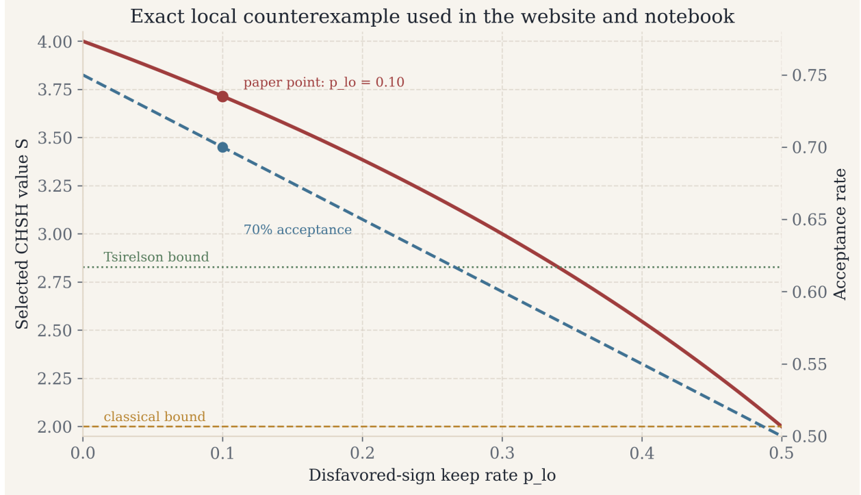
Figure 3: The exact local counterexample used by the revised paper, website widget, and notebook. At p_{lo} = 0.10 , the model yields S = 26/7 with 70.0% acceptance while the underlying source remains local and classical before selection.
