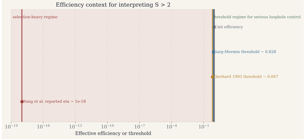
Figure 2: Efficiency context. Wang et al. report an effective efficiency near 10^{-18} , far below the threshold regime usually discussed when one wants detector-loophole-resistant Bell claims [14, 5, 6].
