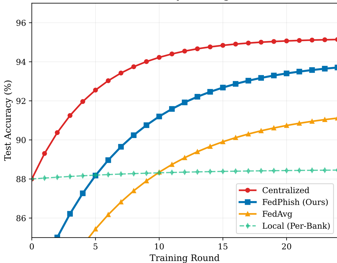
(a) Accuracy Convergence
