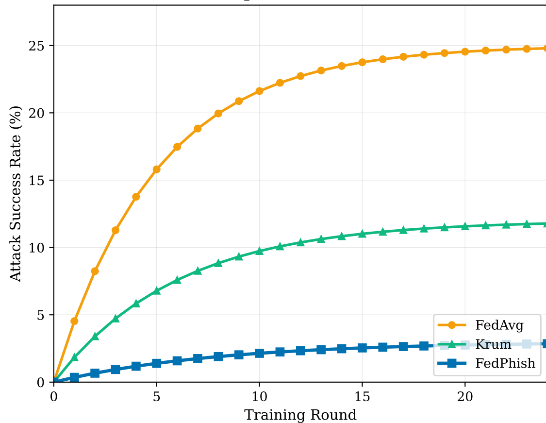
(a) Label Flip Attack (20% Malicious)
