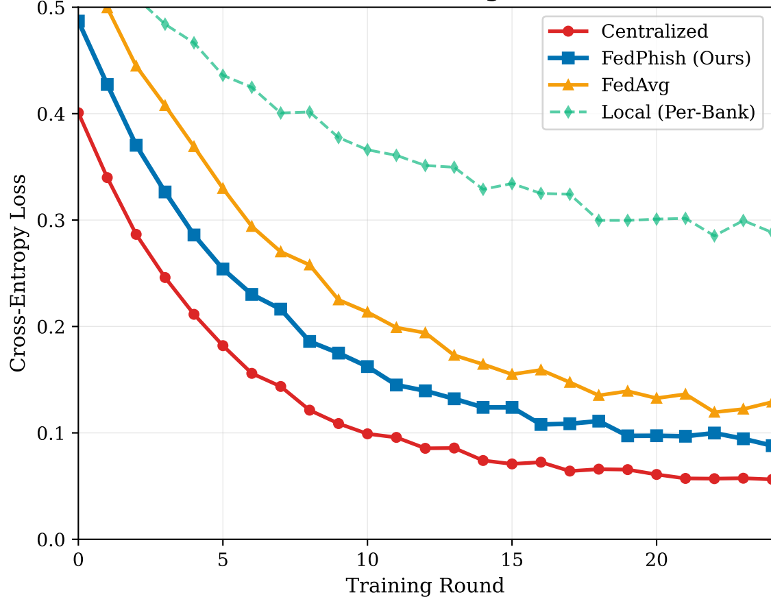
(b) Loss Convergence
