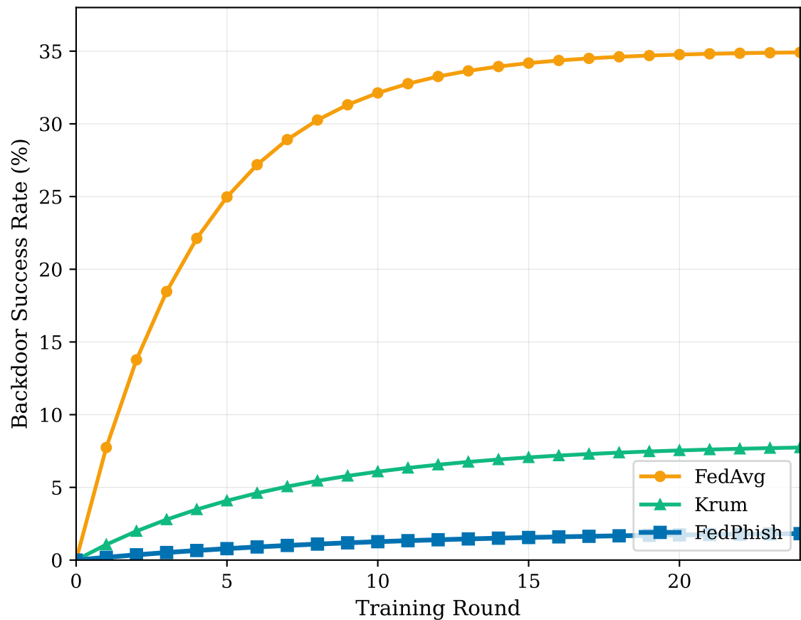
(b) Backdoor Attack (20% Malicious)
