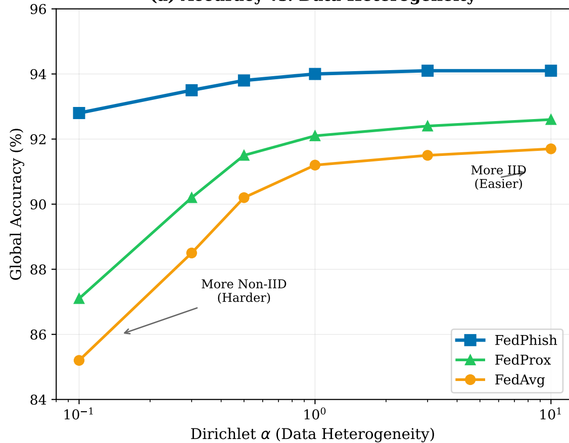
(a) Accuracy vs. Data Heterogeneity
