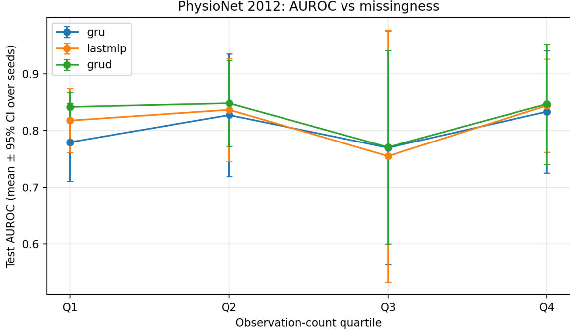
Figure 3: Test AUROC stratified by observation-count quartile (mean \pm 95% CI over 10 seeds), comparing GRU, LastObsMLP, and GRU-D.
