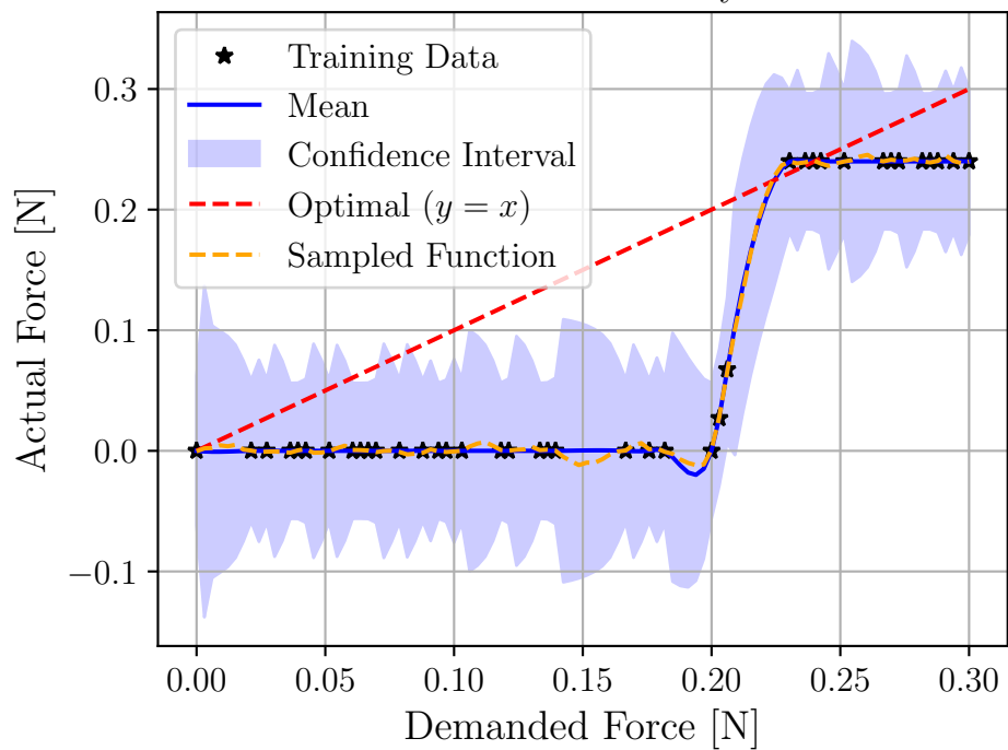
Thruster Failure: Faulty Valve
