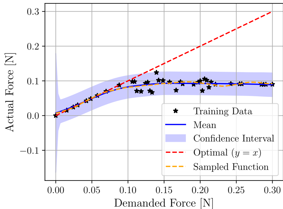
Thruster Failure: Saturated Thrust
