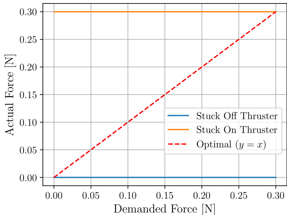
Stuck-Off and Stuck-On Thruster
