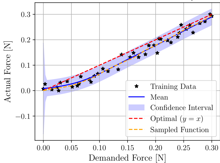
Thruster Failure: Thrust Instability
