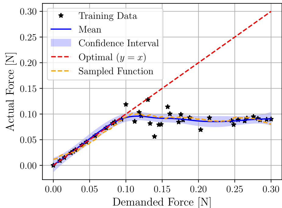
Thruster Failure: Saturated Thrust
