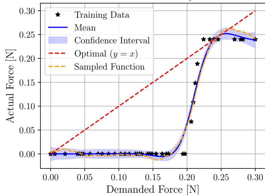
Thruster Failure: Faulty Valve
