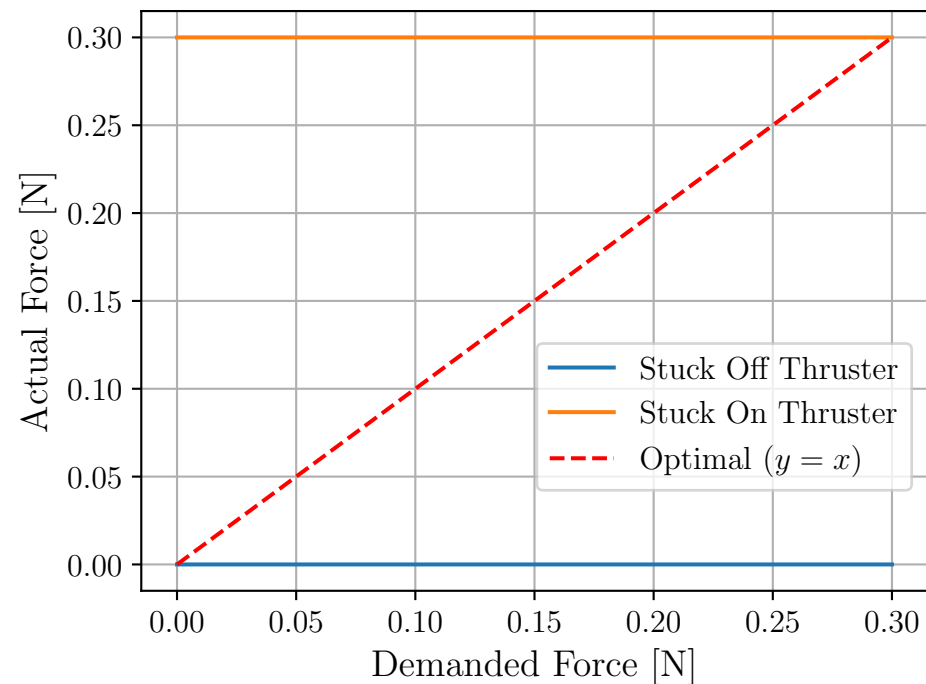
Stuck-Off and Stuck-On Thruster
