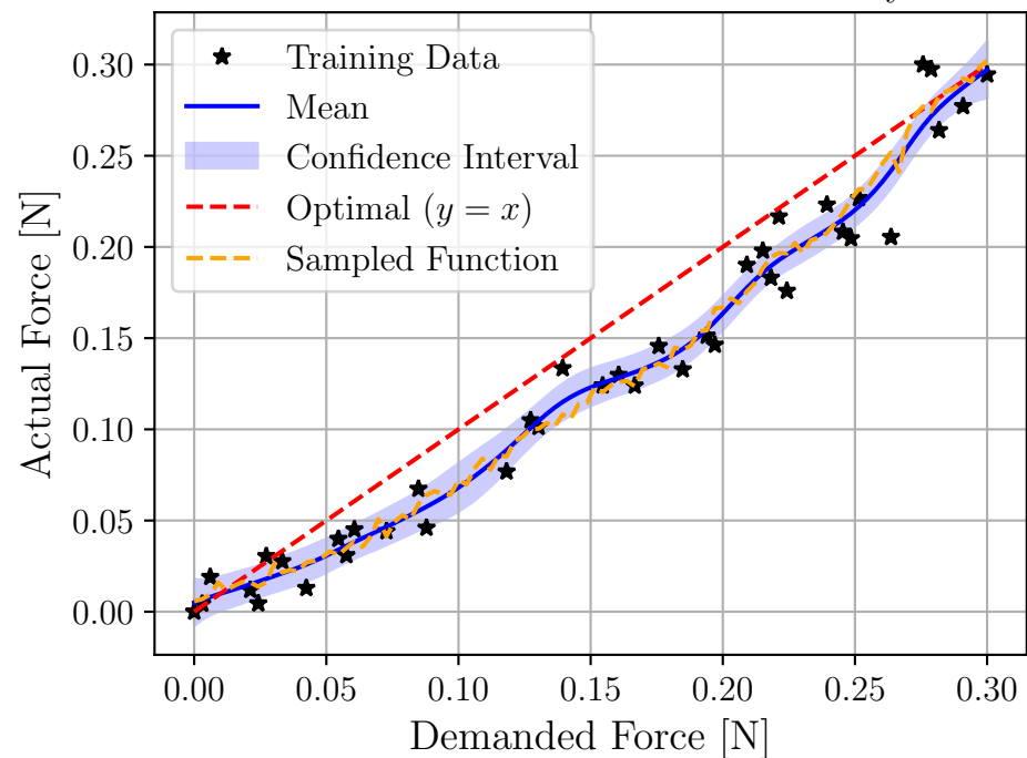
Thruster Failure: Thrust Instability
