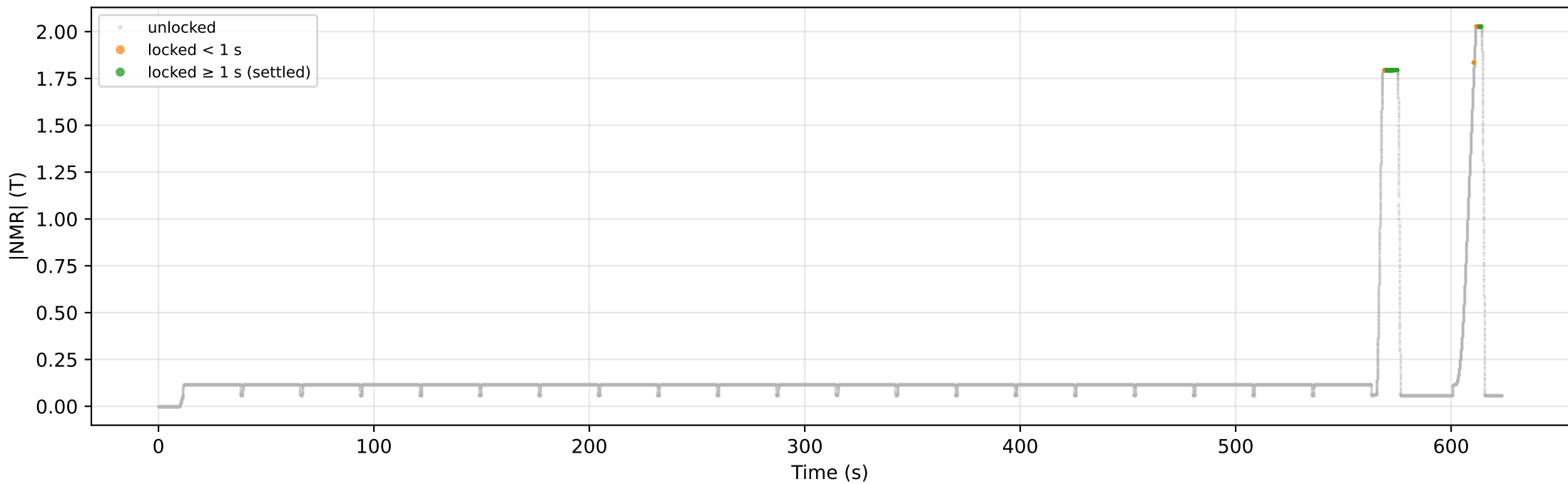
26 GeV — NMR
