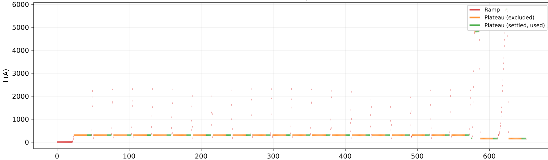
26 GeV — Flattened MD1 (injection only, ~301 A)
