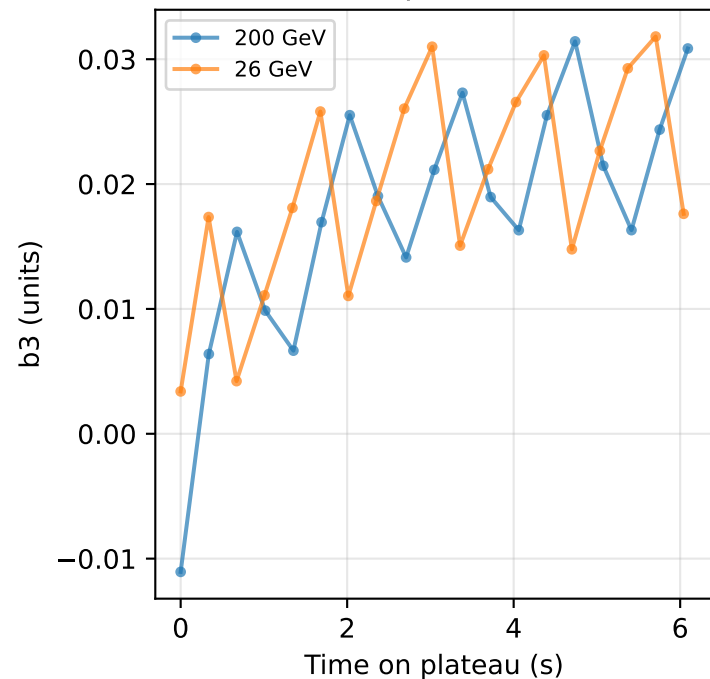
SFTPRO top — b3 (units)
