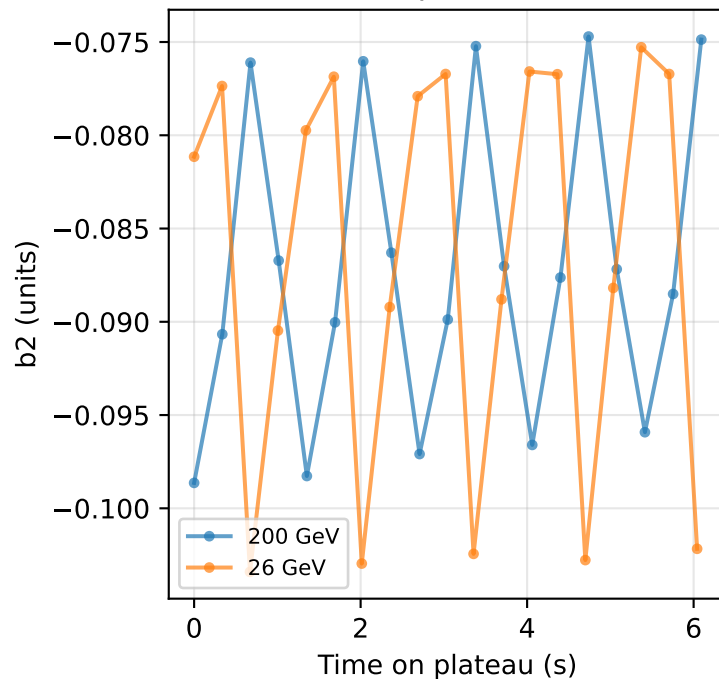
SFTPRO top — b2 (units)
