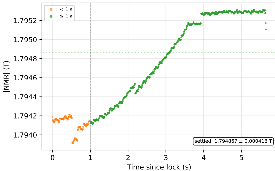
26 GeV — SFTPRO top (5.7 s lock)
