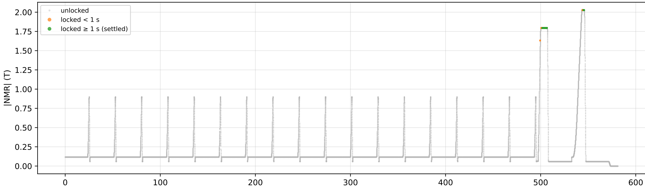
26 GeV — NMR
