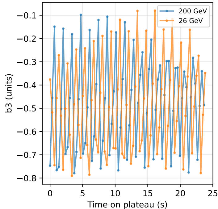
Post-SFTPRO idle — b3 (units)
