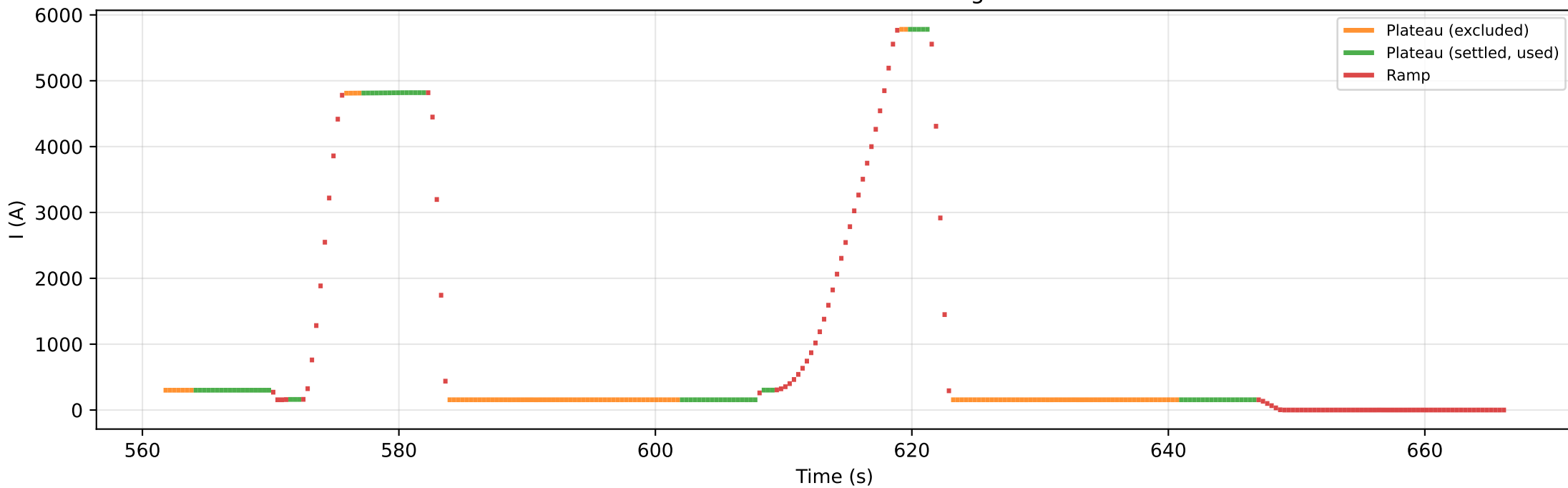
26 GeV — SFTPRO + LHC region
