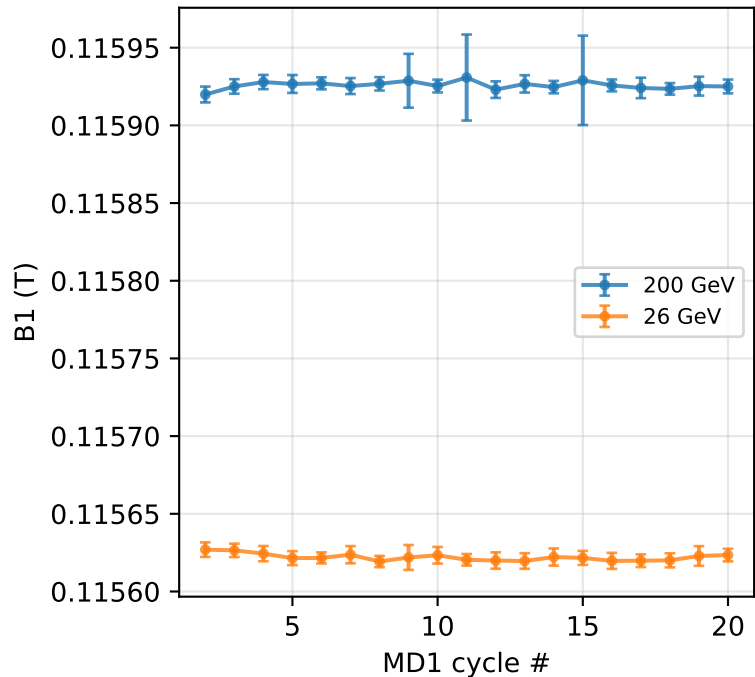
B1 (T) at injection (~301 A)
