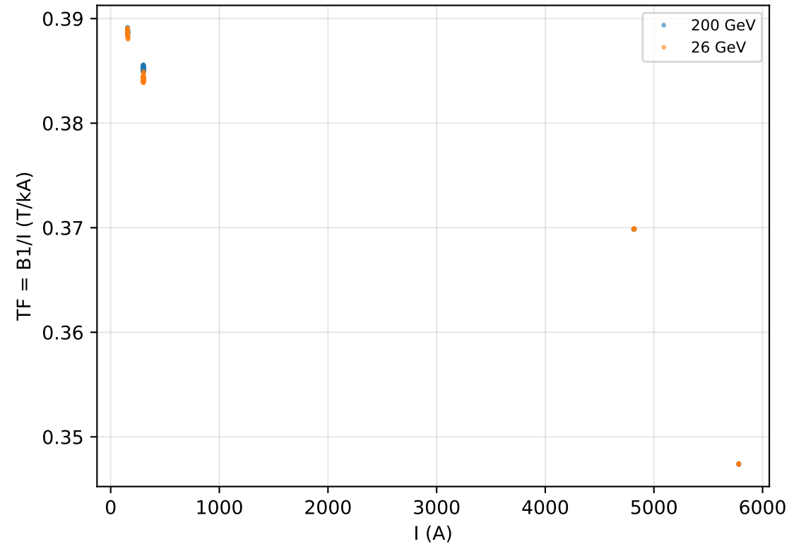
Transfer Function vs Current
