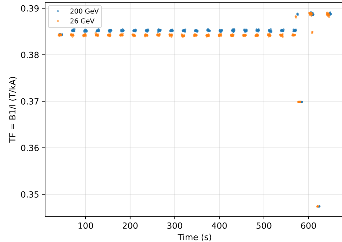
Transfer Function vs Time
