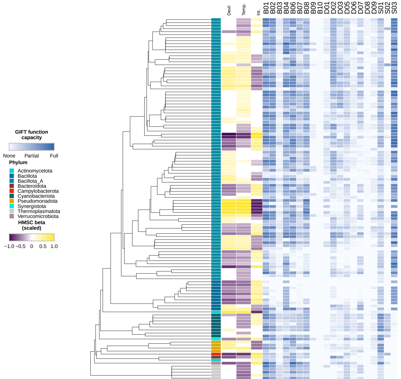
Panels left to right: phylogeny, phylum, HMSC beta (scaled), GIFT function families.
