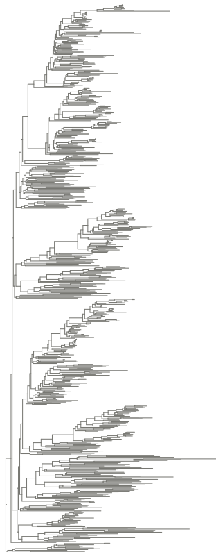
a GTDB bac120 tree
