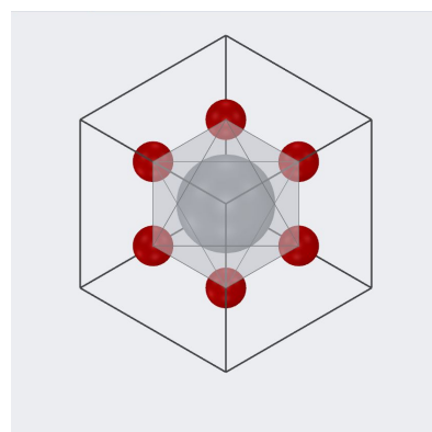
Coordination polyhedron
