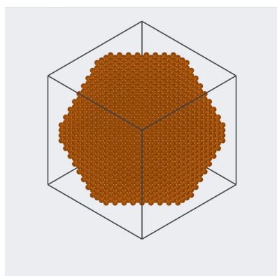
Wulff particle
