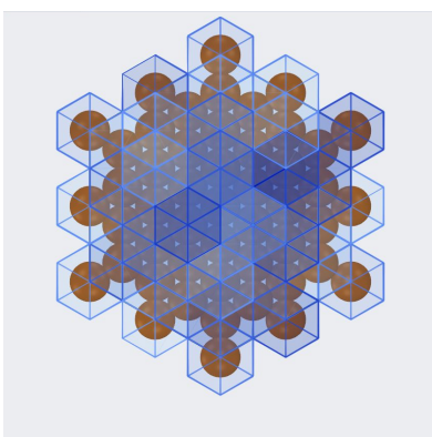
Voronoi cells
