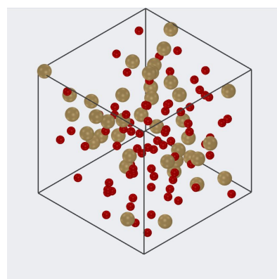
Amorphous packing
