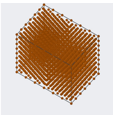
Grain boundary
