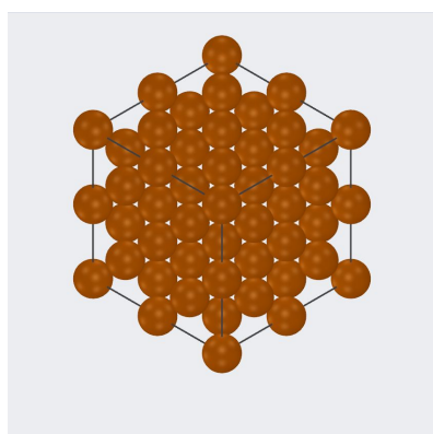
Bulk crystal
