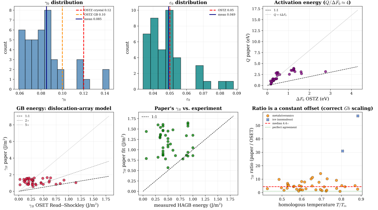
Figure S7: OSET versus Harisankar & Padmanabhan (2025) across all 41 systems. Top row: distributions of the fitted shear eigenstrain \gamma_0 and dilatational eigenstrain \varepsilon_0 against the OSET parameter-free values, and the correlation between the OSET activation barrier \Delta F_0 and the paper's activation energy Q . Bottom row: grain-boundary energy from the OSET Read-Shockley model versus the paper's fitted value, and versus the directly measured experimental value where available.
