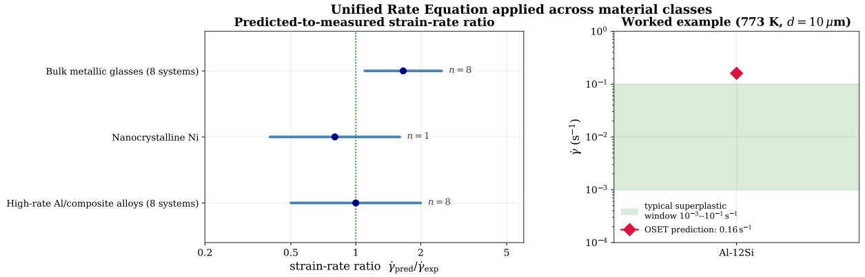
Figure S6: Unified Rate Equation applied across material classes. Left: predicted-to-measured strain-rate ratio \dot{\gamma}_{pred}/\dot{\gamma}_{exp} for the three independent literature compilations of Table S3 (markers: geometric mean of the quoted range; bars: full quoted range; n = number of systems in each compilation; the dotted vertical line marks perfect agreement, ratio = 1). Right: the Al-12Si worked example below, plotted against the typical superplastic strain-rate window 10 -3 –10 -1 s -1 (green band); the prediction 0.16 s -1 sits just above the upper edge of this window.
