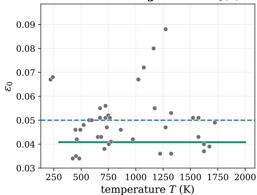
Dilatational eigenstrain \varepsilon_0(T)
