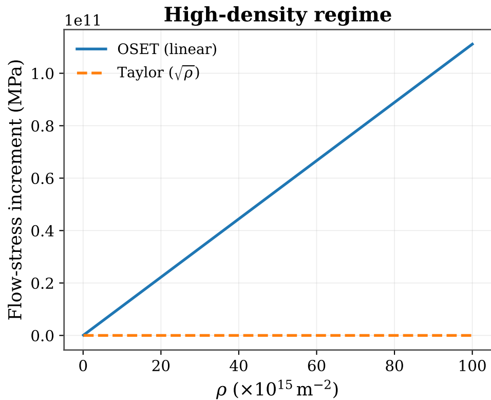
OSET vs. Taylor hardening (Cu, z = 6 )
