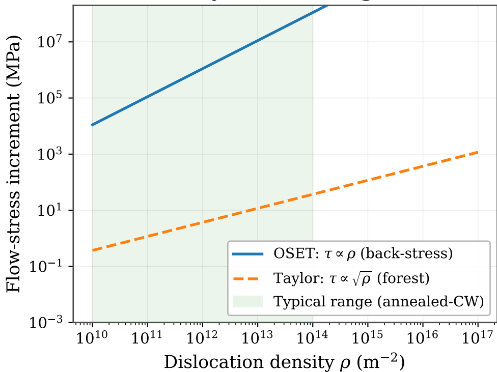
OSET vs. Taylor hardening (Cu, z = 6 )
