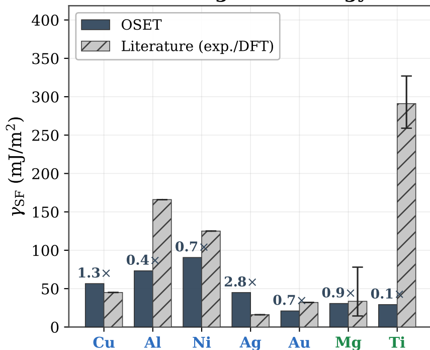
Stacking-fault energy
