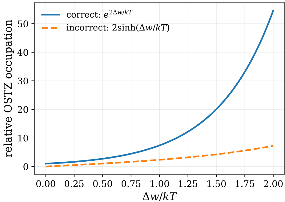
Partition function vs. sinh occupation
