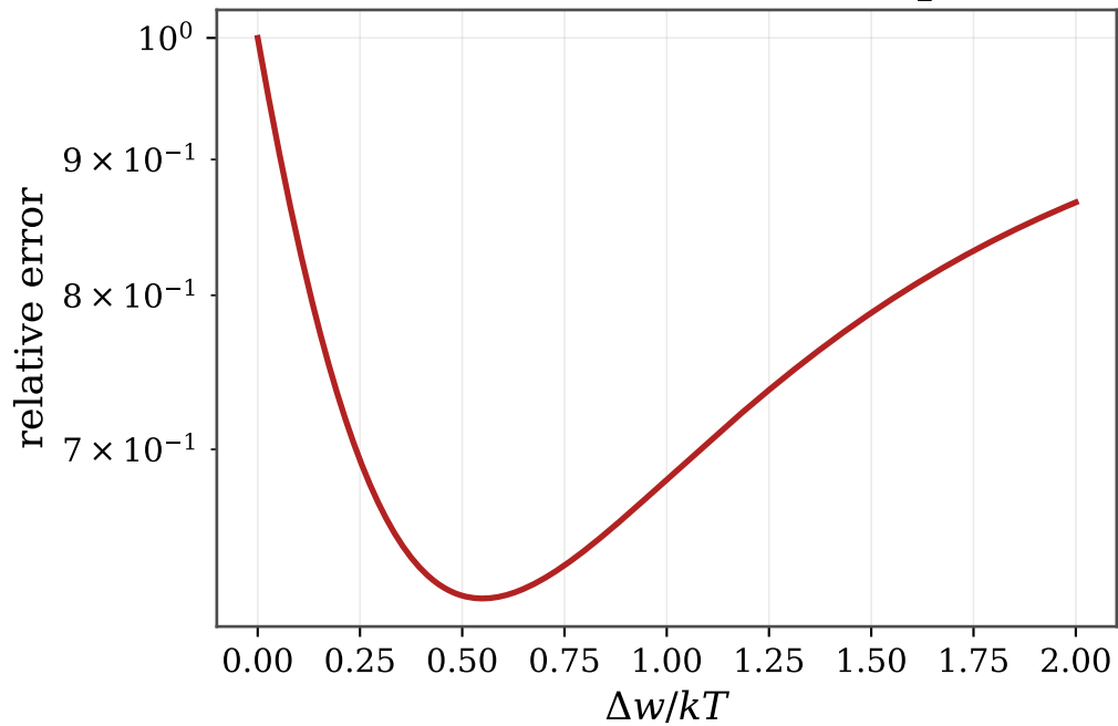
Error of the incorrect sinh expression
