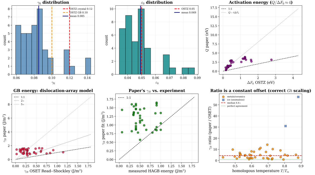
Figure S7: OSET versus Harisankar and Padmanabhan (2025) across all 41 systems. Top row: distributions of the fitted shear eigenstrain \gamma_0 and dilatational eigenstrain \varepsilon_0 against the OSET parameter-free values, and the correlation between the OSET activation barrier \Delta F_0 and the paper's activation energy Q . Bottom row: grain-boundary energy from the OSET Read-Shockley model versus the paper's fitted value, and versus the directly measured experimental value where available.
