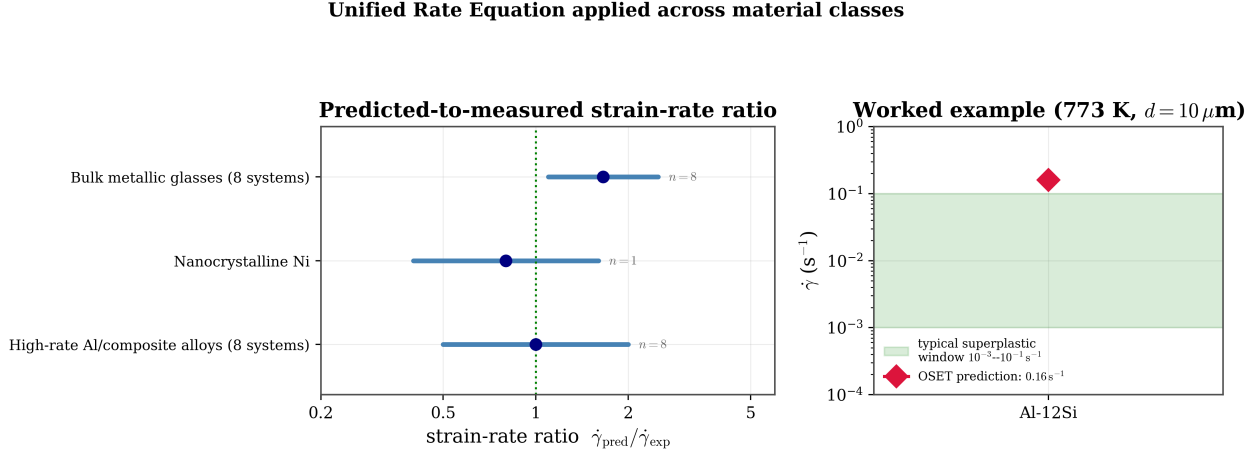
Figure S6: Unified Rate Equation applied across material classes. Left: predicted-to-measured strain-rate ratio \dot{\gamma}_{\text{pred}}/\dot{\gamma}_{\text{exp}} for the three independent literature compilations of Table S3 (markers: geometric mean of the quoted range; bars: full quoted range; n = number of systems in each compilation; the dotted vertical line marks perfect agreement, ratio = 1). Right: the Al-12Si worked example below, plotted against the typical superplastic strain-rate window 10 -3 –10 -1 s -1 (green band); the prediction 0.16 s -1 sits just above the upper edge of this window.
