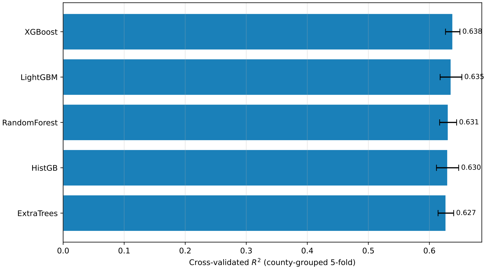
Learner comparison (R3.8) all learners share the same 193 satellite features and CV protocol
